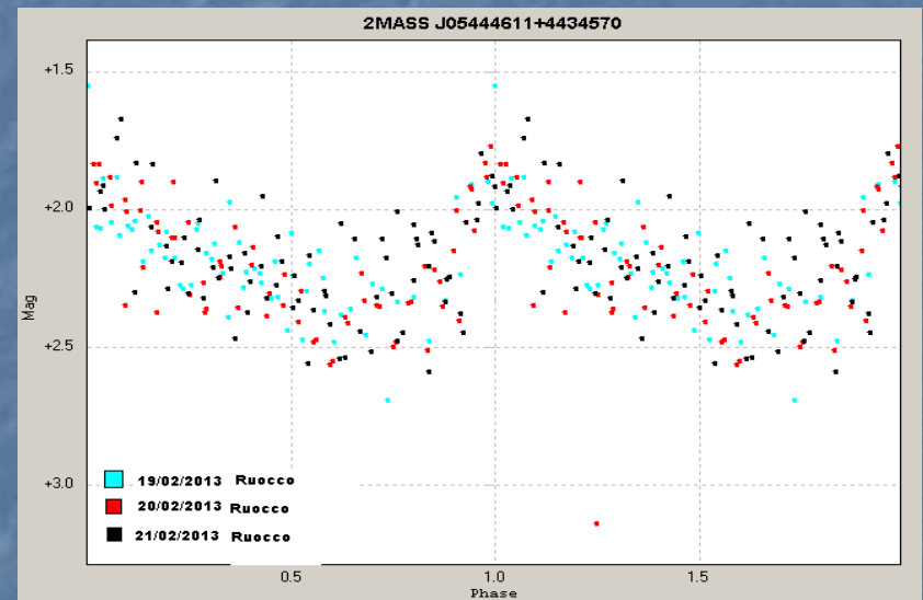
2MASS J05444611+4434570
