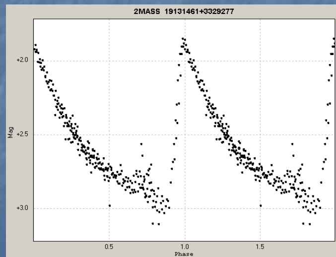
2MASS J19131461+3329277
