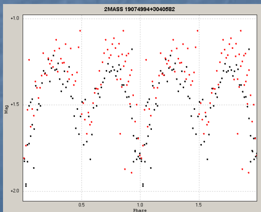
2MASS J19074994+3040582
