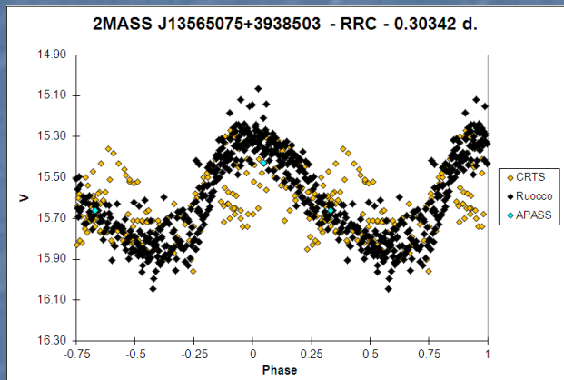
2MASS J13565075+3938503
