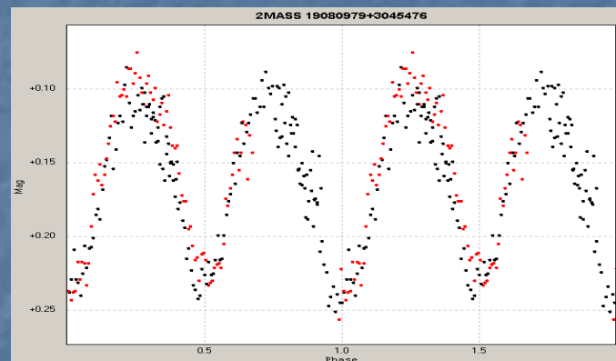
2MASS J19080979+3045476
