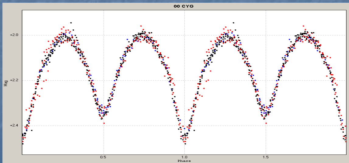
2MASS J19524346+3756501
