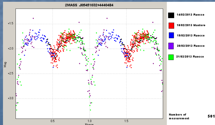
2MASS J05451032+4440484
