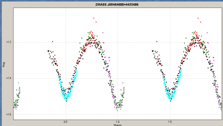
2MASS J05464688+4433486
