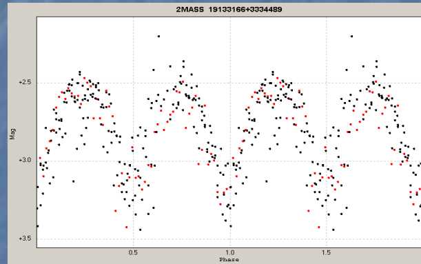
2MASS J19133166+3334489
