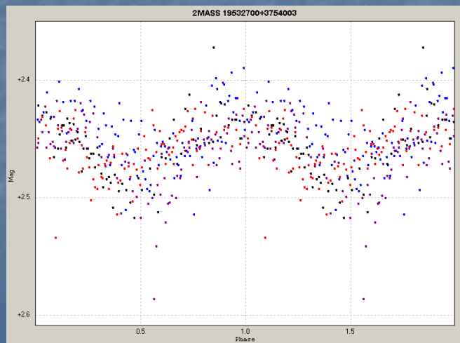
2MASS J19532700+3754003
