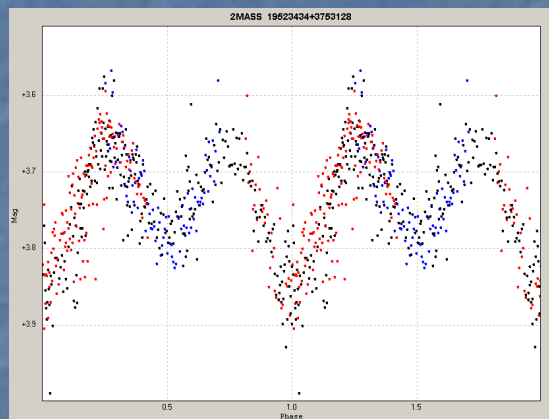
2MASS J19523434+3753128
