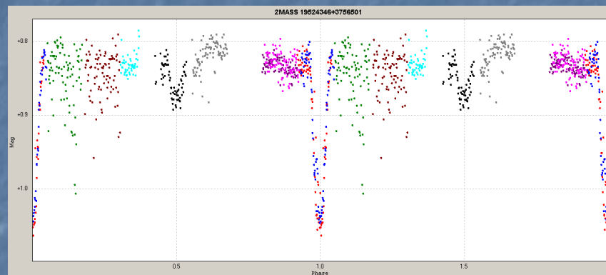
2MASS J19524346+3756501
